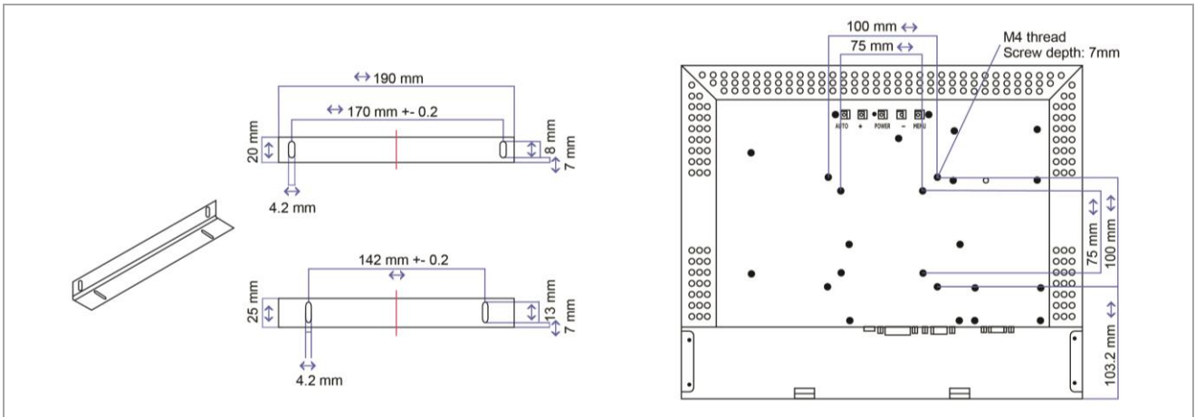
Figure 4: Standard L-Brackets and VESA Mount
