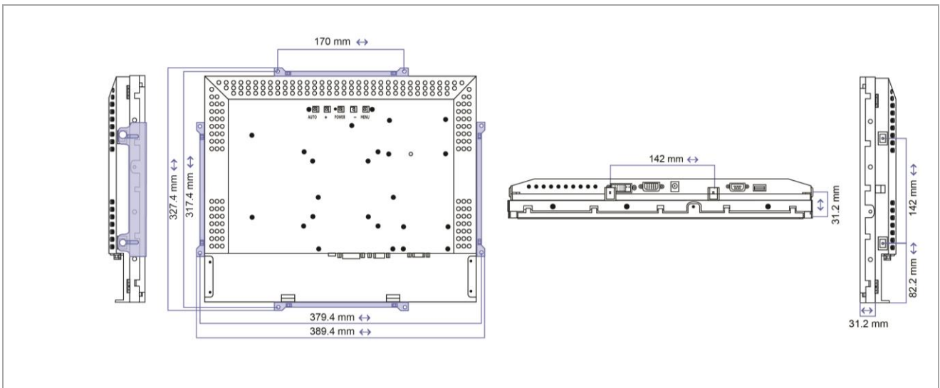
Figure 3: Monitor with Standard L-Brackets
