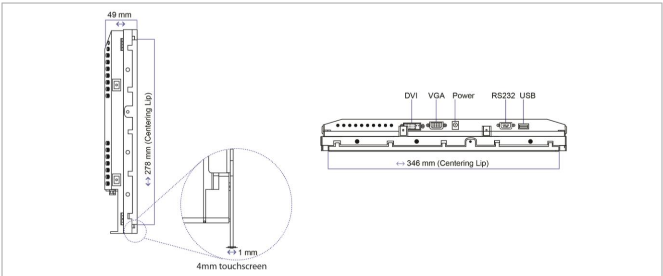
Figure 2: Monitor Side View
